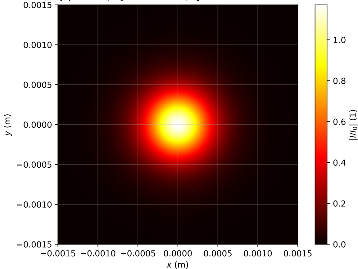
Intensity profile I(x, y, z = 2.707m)/I_0 , Pin=0.8Pcr, artificial time
